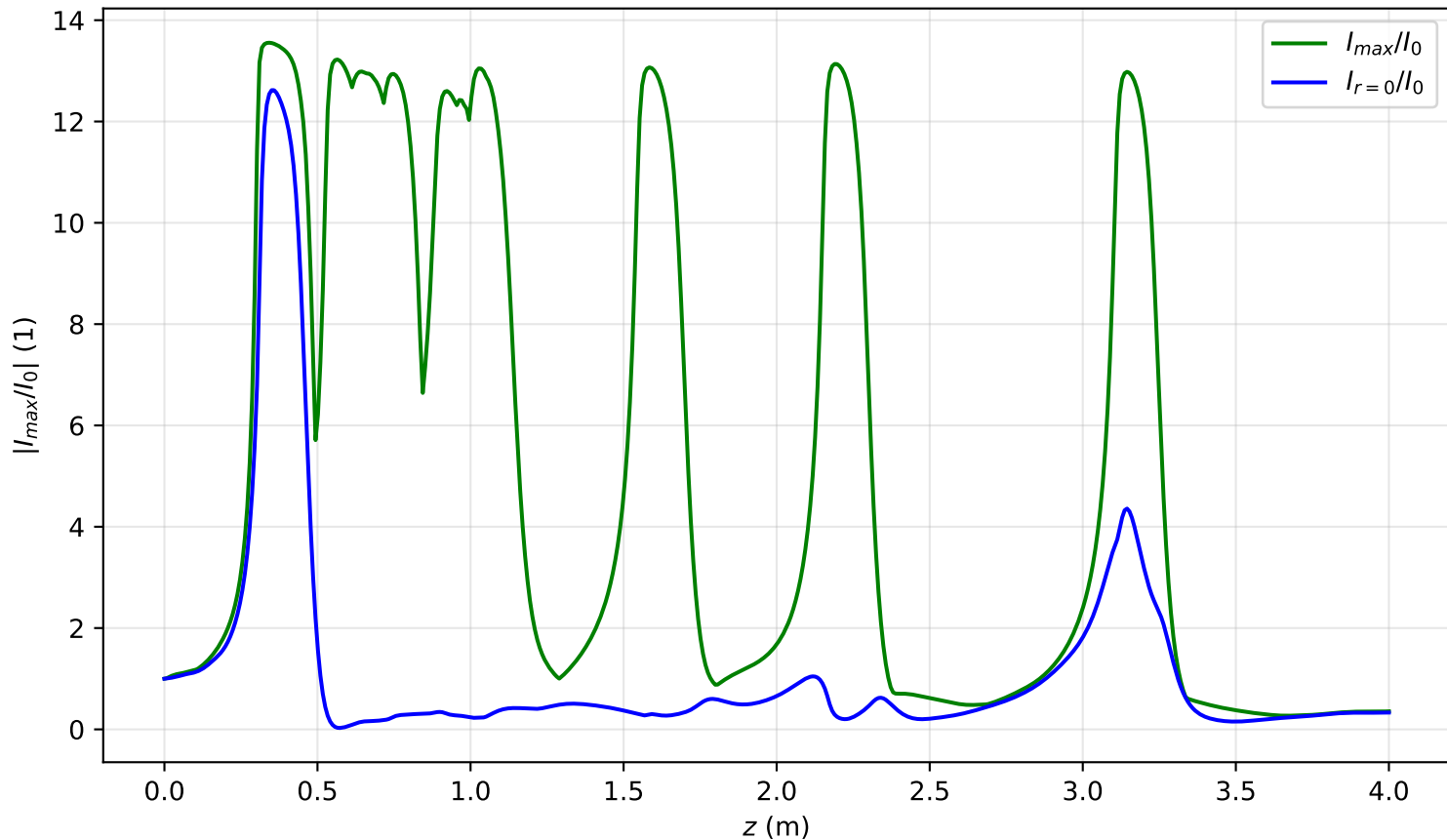
I_{max}(x=0, y=0, z)/I_0 , \text{Pin}=8.2\text{Pcr} , noisy input, artificial time
